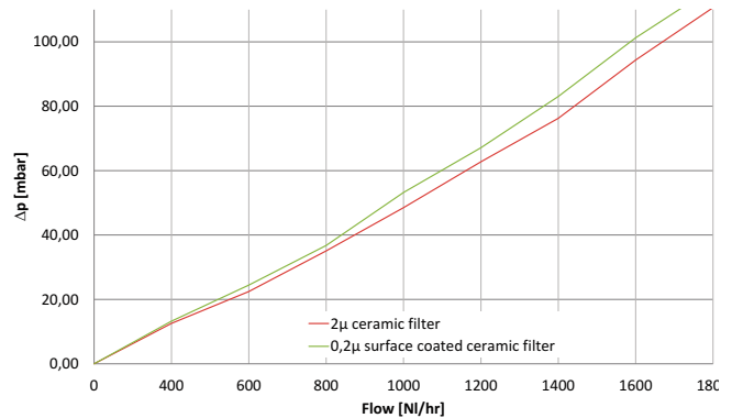
Pressure characteristics in dependence of the gas flow (for new filter element and 20°C)
